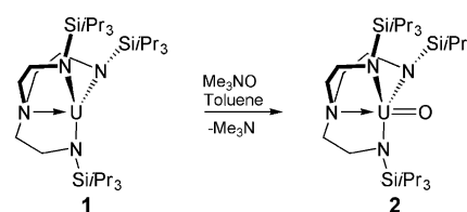
Scheme 1. Synthesis of 2 .
